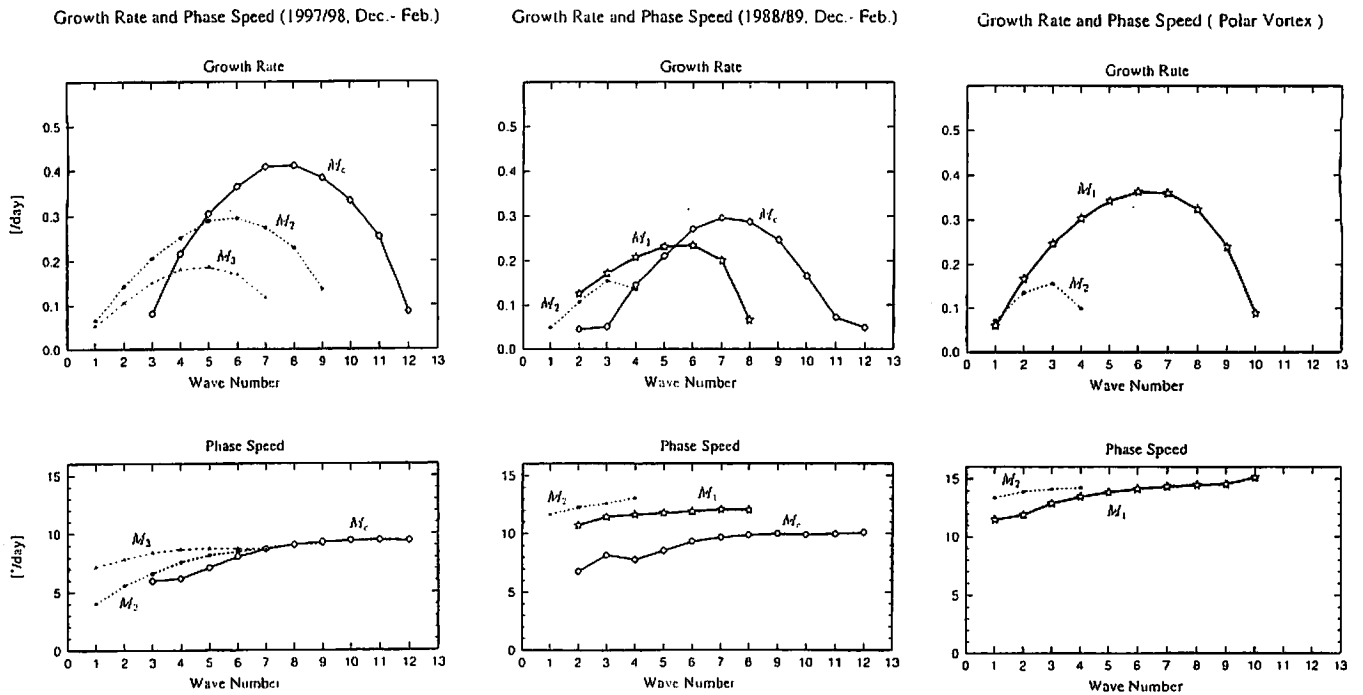
Fig. 2 Growth rates ( \text{day}^{-1} ) and phase speeds ( ^{\circ}\text{day}^{-1} ) of the unstable modes for the zonal mean basic state of (a) weak polar vortex, (b) strong polar vortex, and (c) hypothetical zonal mean zonal wind shown in Fig. 1. The unstable modes are labeled M_C for shallow Charney modes, M_2 for dipole Charney modes, M_3 for tripole Charney modes, and M_1 for monopole Charney modes.
