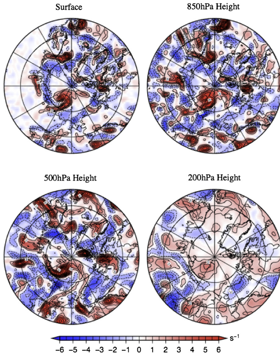
Fig. 5. Same as Fig. 3, but for the Case 3. (For interpretation of the references to color in this figure legend, the reader is referred to the web version of this article.)
