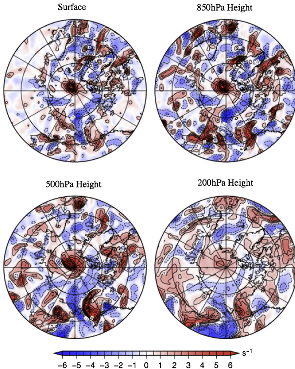
Fig. 3. Scaled relative vorticity for the Case 1 at SLP (top left), 850 hPa height (top right), 500 hPa height (bottom left) and 200 hPa height (bottom right). The red and blue colors show positive and negative vorticity, respectively. (For interpretation of the references to color in this figure legend, the reader is referred to the web version of this article.)
