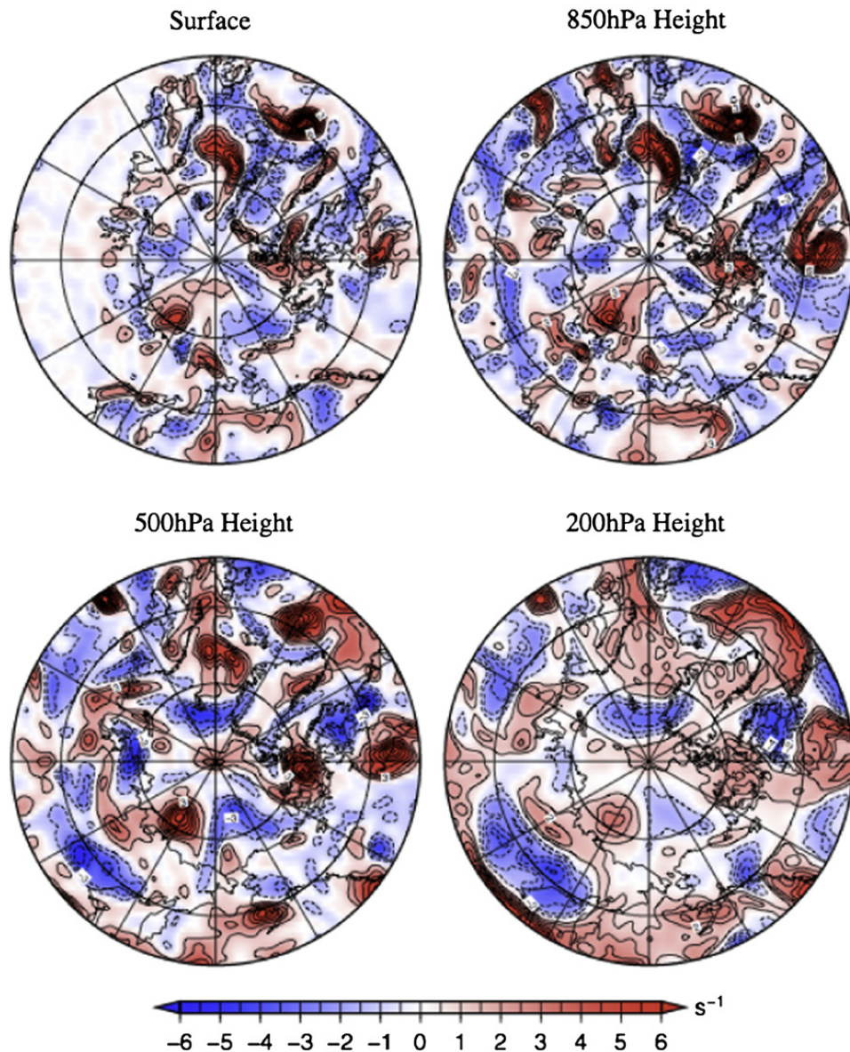
Fig. 4. Same as Fig. 3, but for the Case 2. (For interpretation of the references to color in this figure legend, the reader is referred to the web version of this article.)
