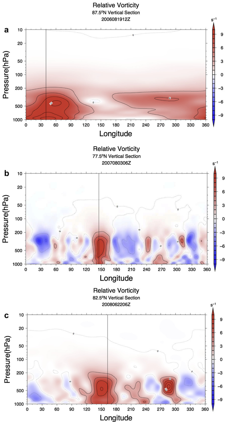
Fig. 9. Longitude-height cross section of scaled relative vorticity. Cyclone center is marked by a line at 40°E in Case 1 (a), 145°E in Case 2 (b) and 162.5°E in Case 3 (c). The values are scaled in colors. (For interpretation of the references to color in this figure legend, the reader is referred to the web version of this article.)
